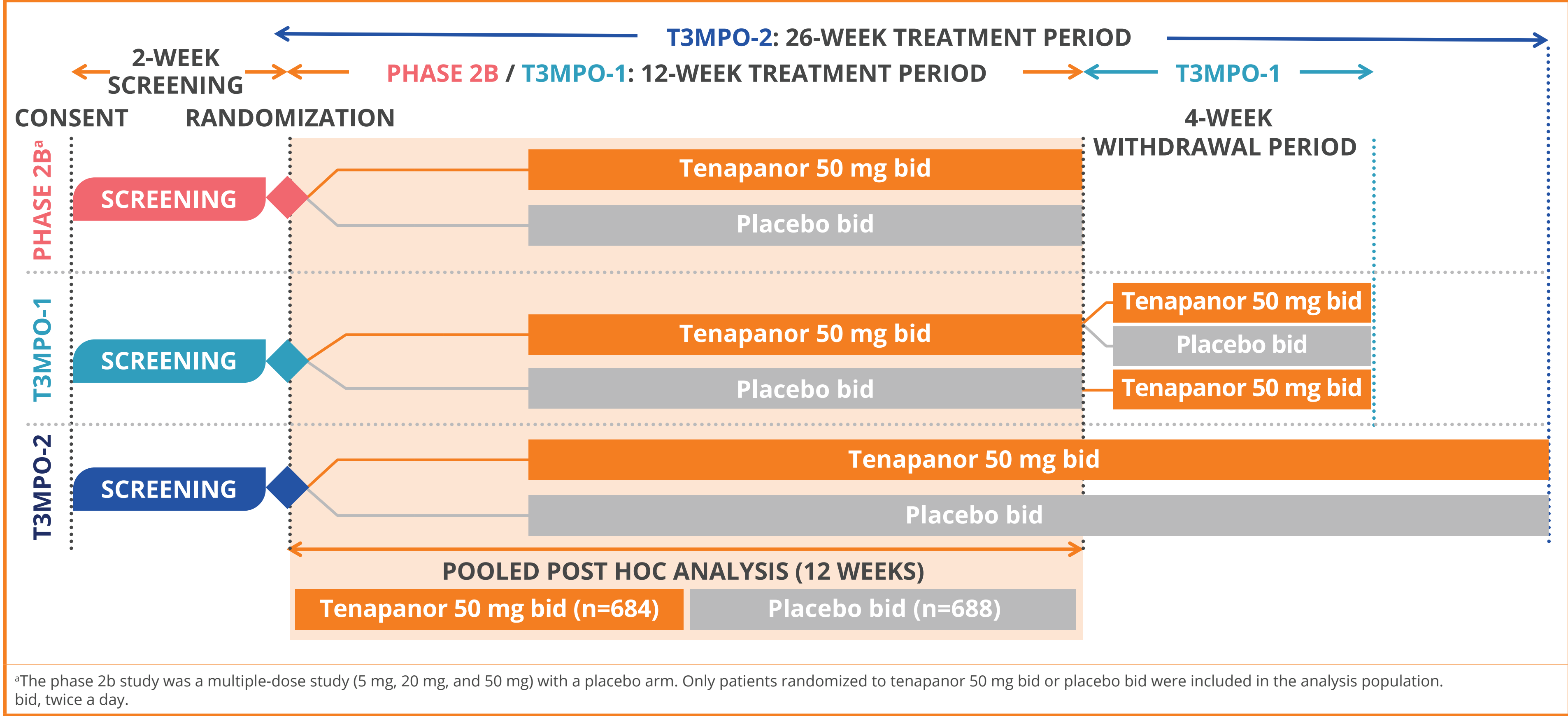
Figure 1. Study Design
